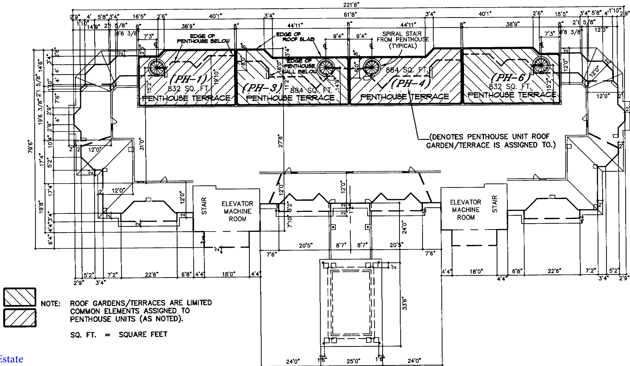
ROOF PLAN
