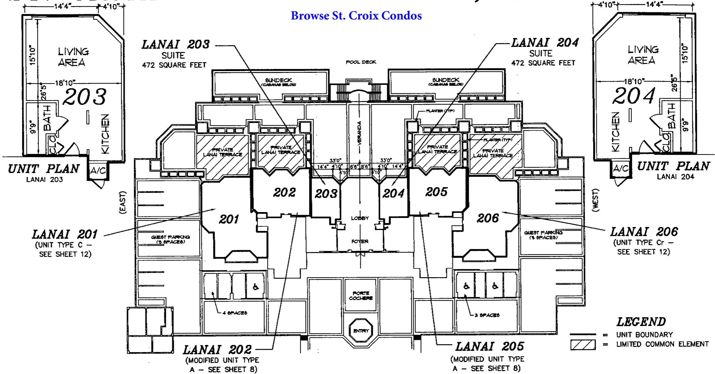
LOBBY LEVEL FLOOR PLAN
